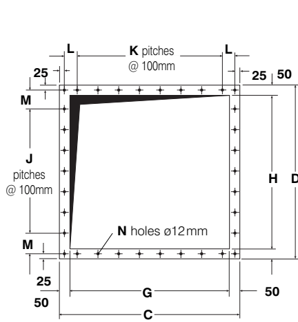
Vertical upstand base flange details for all filters except DLM V30/10 and V21/7
